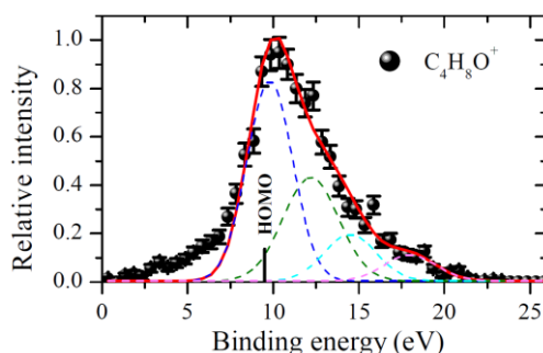
Figure 2. (e,2e+ion) binding energy spectrum for the C_4H_8O^+ ion of tetrahydrofuran for 35 eV electron impact. The dashed lines are the fitted Gaussian peaks.
